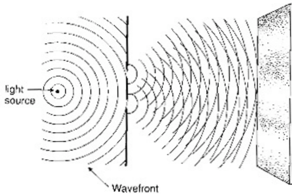
Light interference in a double-slit apparatus.
